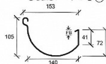
ROOFING INDUSTRIES 153mm HALF ROUND FLAT BACK GUTTER
