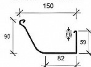
ROOFING INDUSTRIES QUARTER ROUND GUTTER
