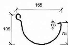
ROOFING INDUSTRIES 155mm HALF ROUND GUTTER
