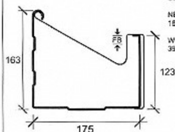
ROOFING INDUSTRIES 175 BOX GUTTER WITH INTERNAL BRACKET
