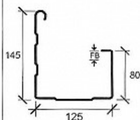
ROOFING INDUSTRIES 125 BOX GUTTER
