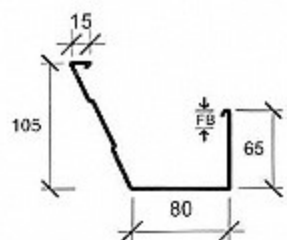
ROOFING INDUSTRIES J LINE GUTTER
