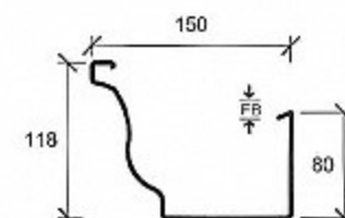
ROOFING INDUSTRIES 150mm OLD GOTHIC GUTTER
