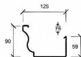
ROOFING INDUSTRIES 125mm OLD GOTHIC GUTTER
