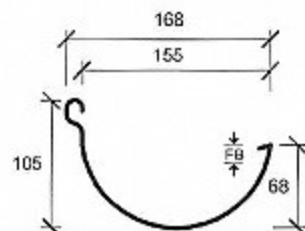
ROOFING INDUSTRIES 168mm HALF ROUND GUTTER
