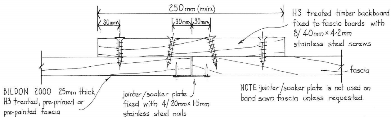
PLAN VIEW
