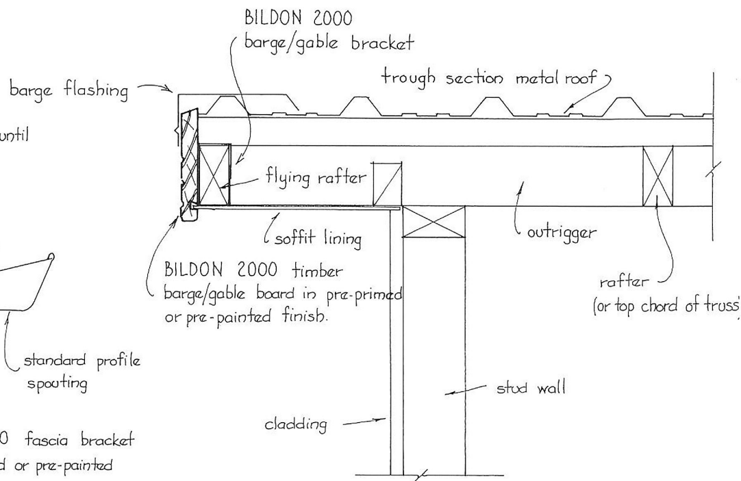
BARGE
