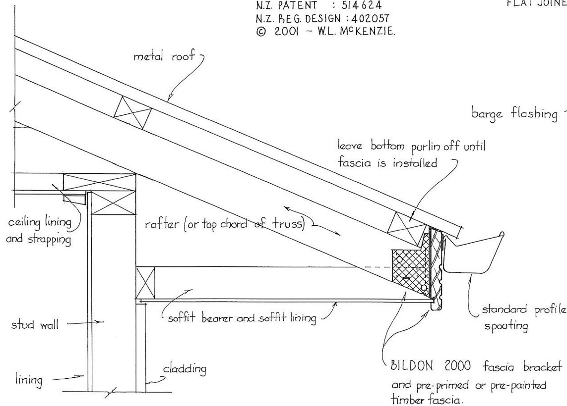
EAVES
